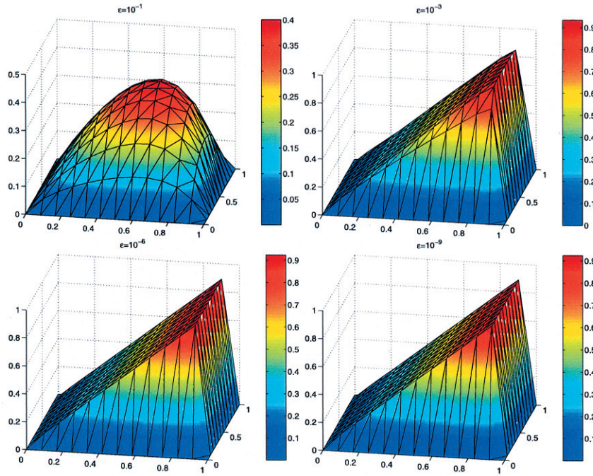
FIGURE 9. Solution for the bubble test case using structured meshes for different values of \varepsilon .
