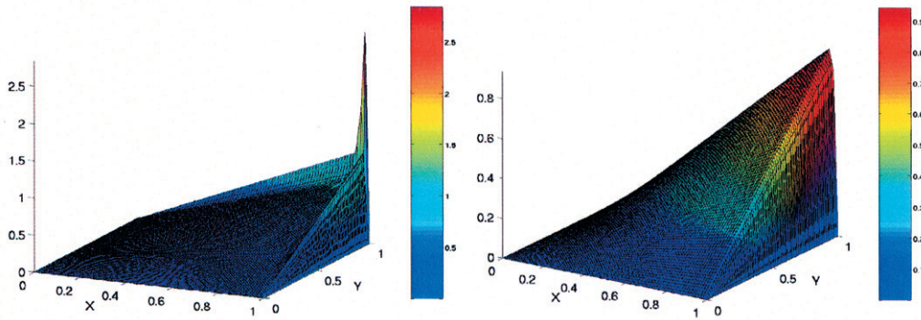
FIGURE 12. Solutions for h = 1/80 and \varepsilon = 10^{-3} . Plain formulation (left) and stabilized formulation (right).
