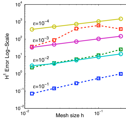
FIGURE 11. Error curves as functions of h and for different values of \varepsilon . Dashed line: plain DPG method, solid line: flux-upwind stabilized scheme.
