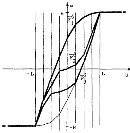
Figure 9. — Piecewise linear monotone curves in the (u, w) -plane corresponding to the graphs B_1, B_2 and B_3 shown in figure 8, in the case \mu = Lebesgue measure.
