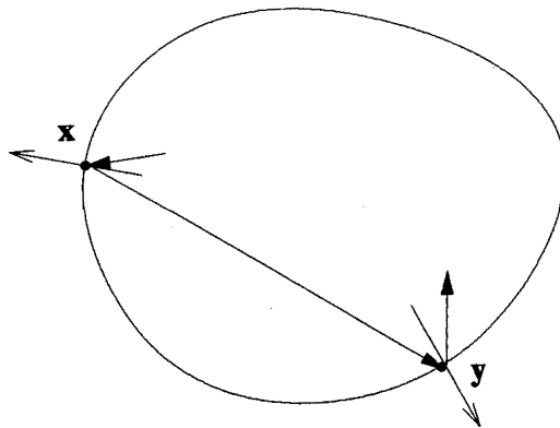
Figure 5. — Reflection in x , transmission in y .
