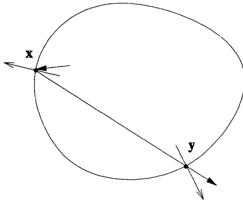
Figure 6. — Reflection in x , reflection in y .
