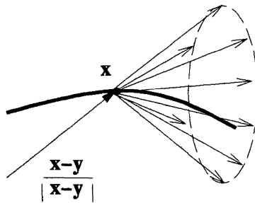
Figure 7. — Stationary phase on a line.
