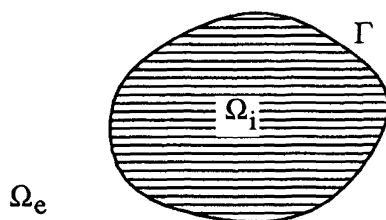
Figure 1. — Position of the problem.
