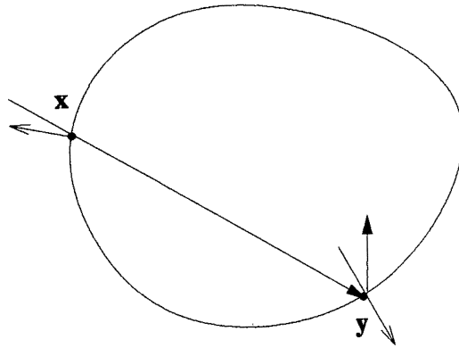
Figure 4. — Transmission in x , reflection in y .
