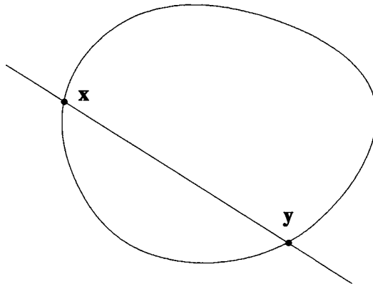
Figure 3. — Transmission in x , transmission in y .
