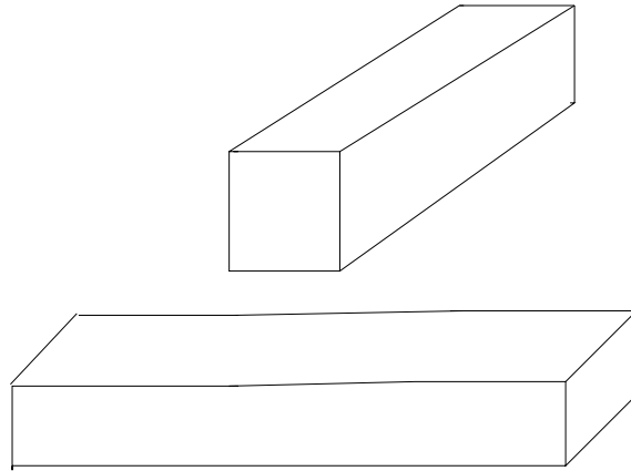
FIGURE 2. Domain decomposition with regular bounded subdomains.
