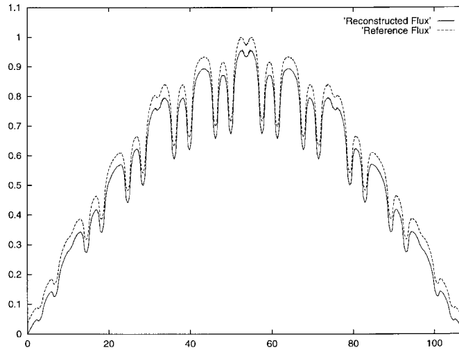
FIGURE 1. Reference flux and reconstructed flux in a core composed of 5 \times 5 assemblies.
