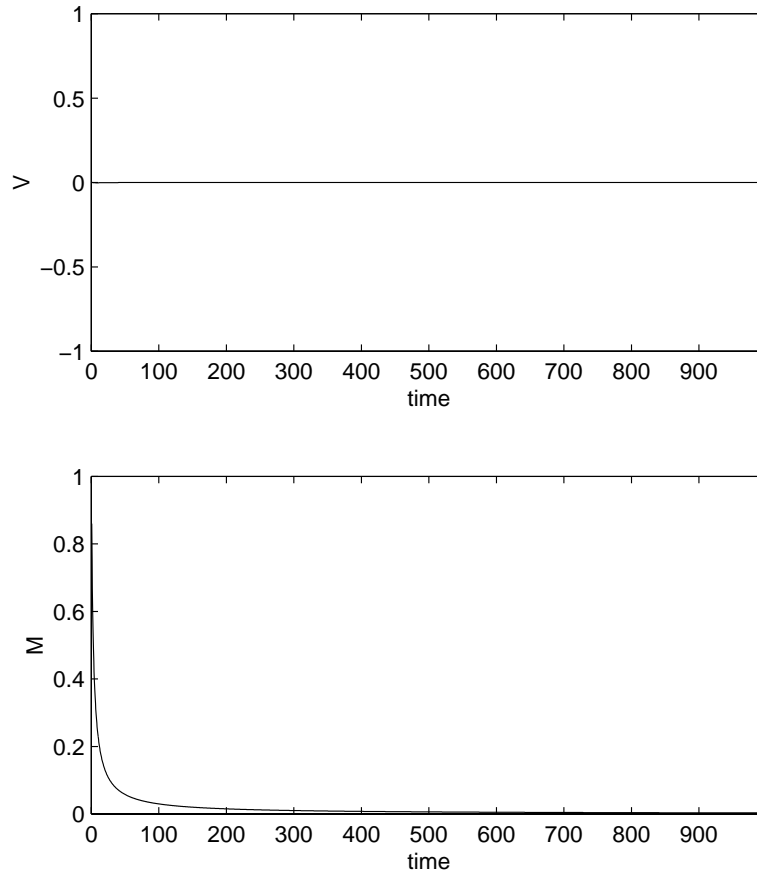
FIGURE 7. The conservation of V(t) and the decay of the M(t) in time.
