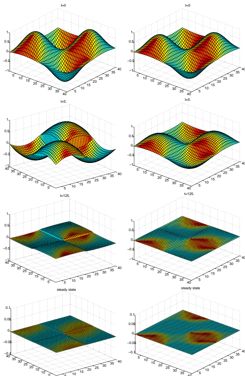
FIGURE 6. The time evolution of the vorticity \omega (left) and the magnetic field u (right).
