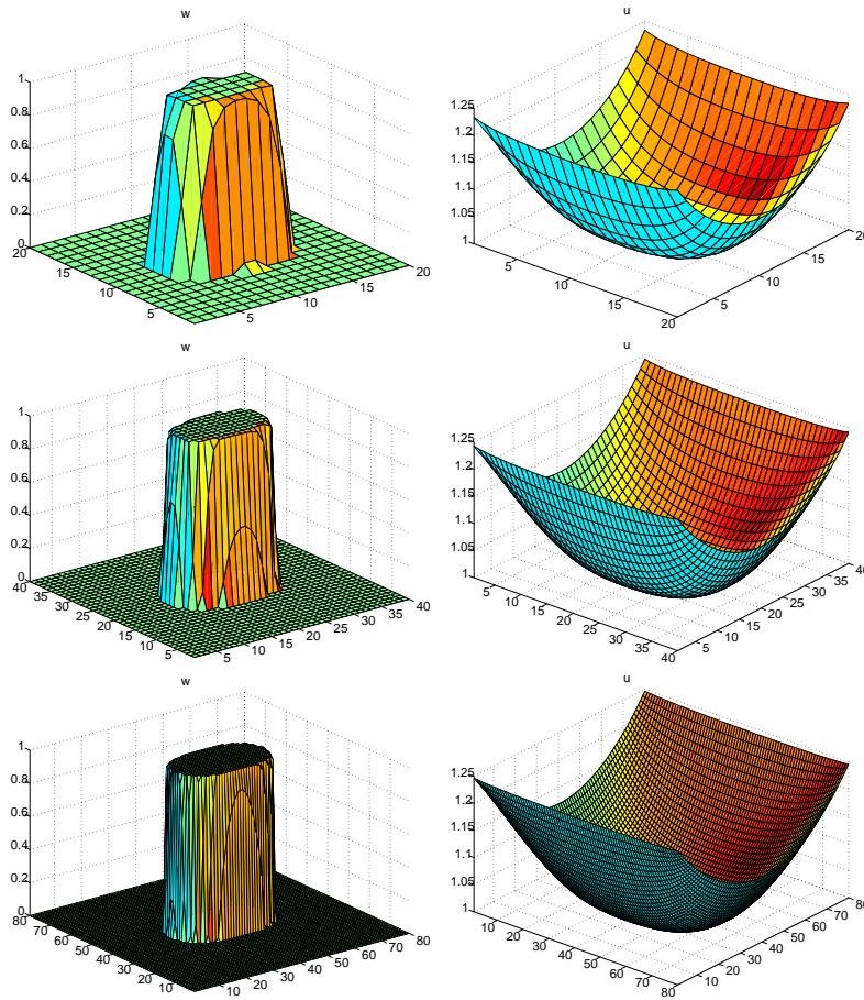
FIGURE 2. The steady state vortex densities (left) and the magnetic fields (right): h = 1/10, 1/20, 1/40 .
