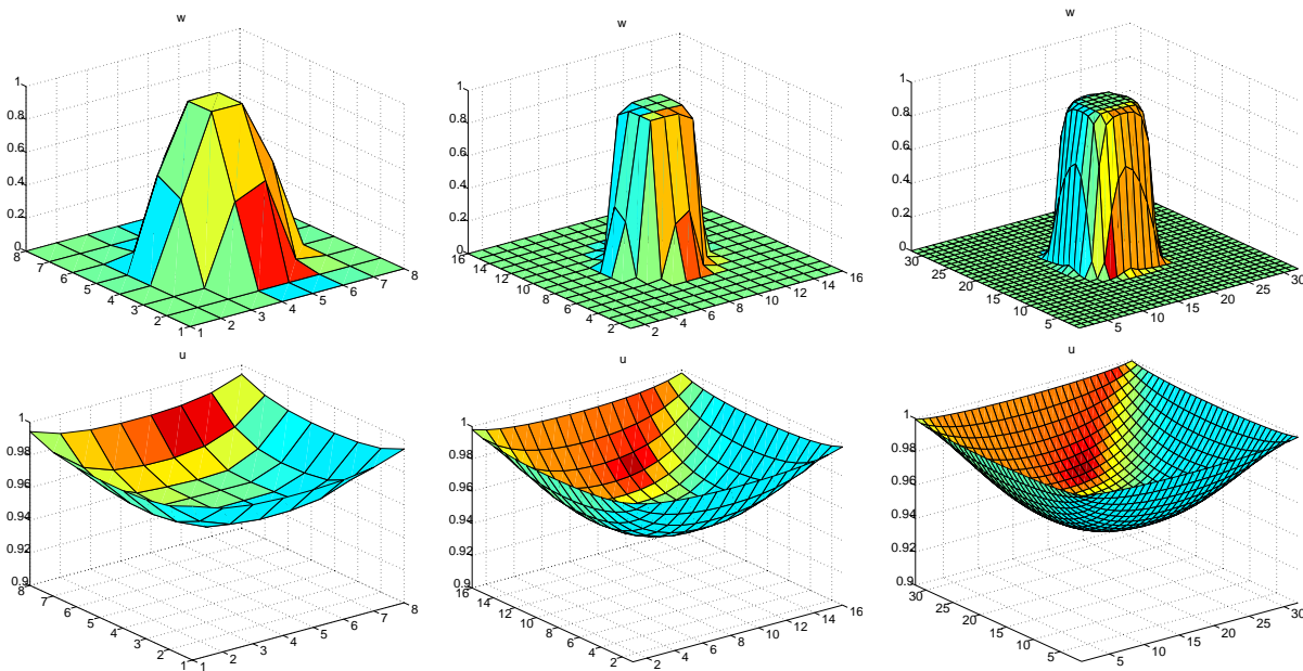
FIGURE 1. The steady state vortex densities (top) and the magnetic fields (bottom): h = 1/8, 1/16, 1/32 .
