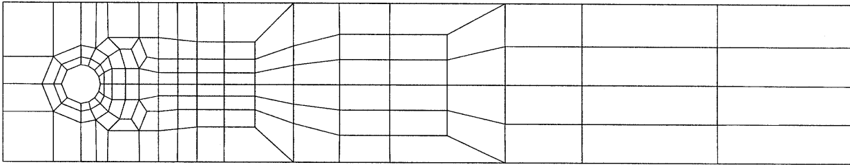
FIGURE 3. Coarse grid partition for non-conforming FE.
