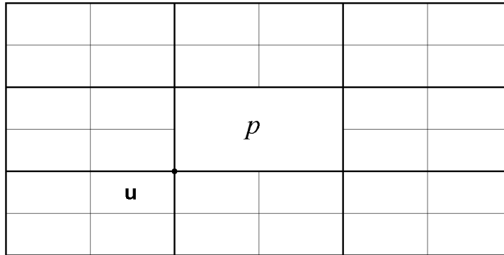
FIGURE 2. (Q^1_{h/2})^2 \times Q^0 velocity-pressure FE.
