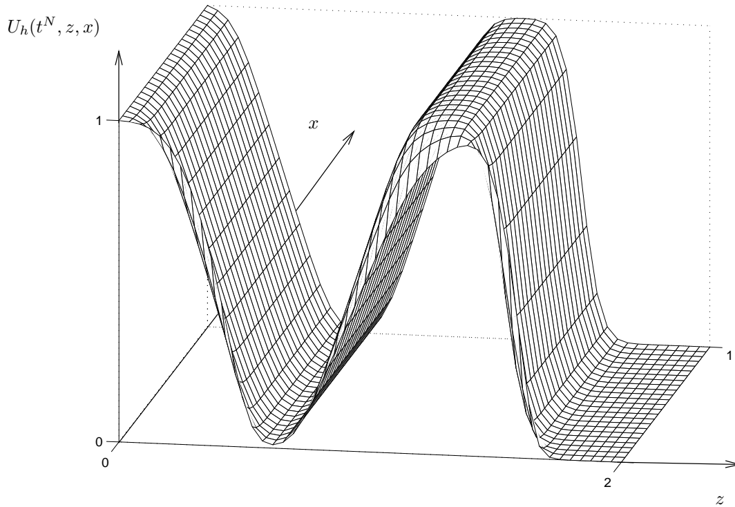
FIGURE 5. Numerical solution for K = 3 .
