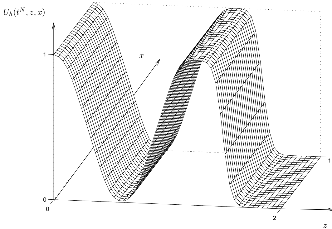
FIGURE 4. Numerical solution for K = 0 .
