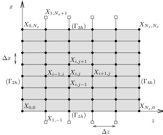
FIGURE 2. The grid.
