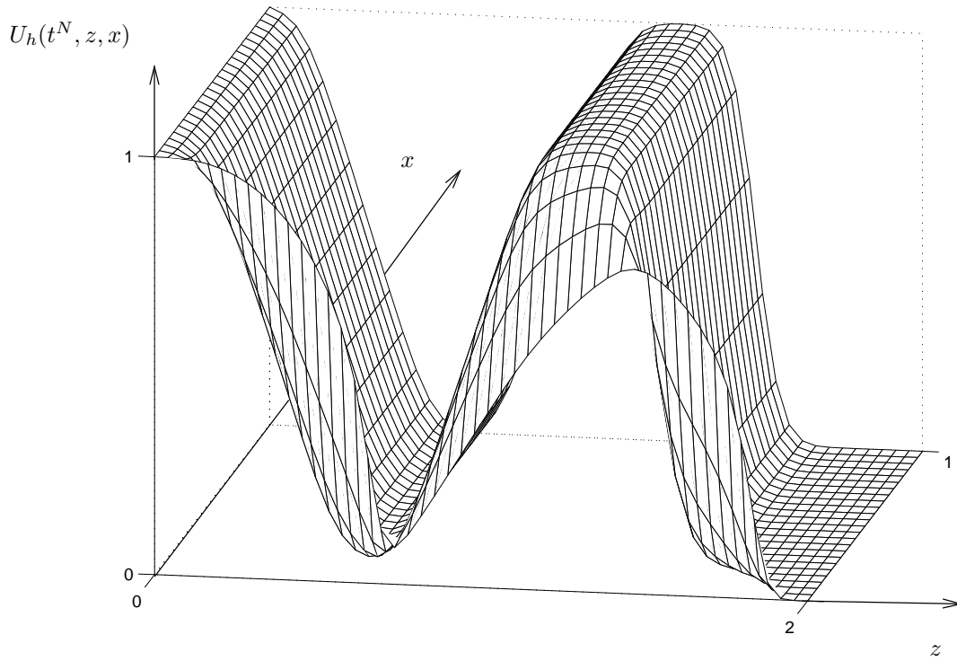
FIGURE 6. Numerical solution for K = 10 .
