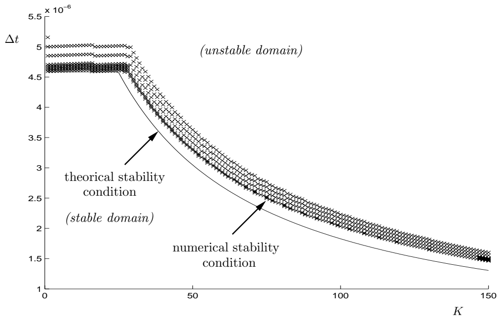
FIGURE 7. Stability of the scheme.
