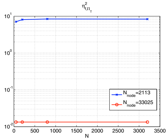
FIGURE 12. Test Problem 1: \eta_{f,\Pi_T}^2 for different timesteps.
