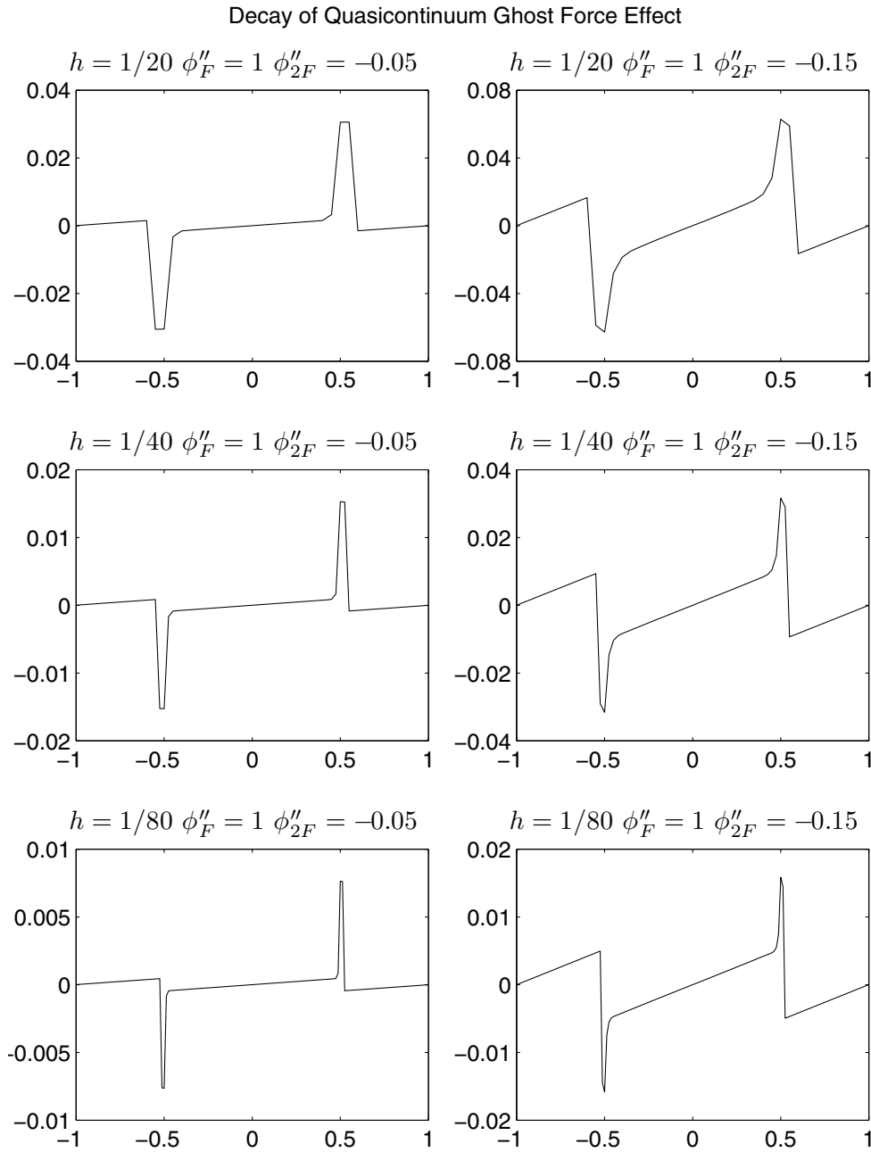
FIGURE 1. Error for the energy-based quasicontinuum approximation, \mathbf{u}_{qc} . We observe that the magnitude of the error is O(h) . However, the oscillation near the interface means that the error in the displacement gradient is O(1) in the interfacial region. The average deformation gradient, F , for the right column is close to failing the stability condition \phi''_F + 5\phi''_{2F} > 0 . In all plots K = N/2 and \phi'_{2F} = 1 .
