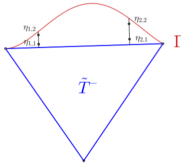
FIGURE C.1. Illustration of the Gauss points.
