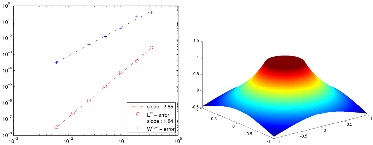
FIGURE 2. Plot of the L^\infty and W^{1,\infty} errors (left) and the approximate solution (right) by method (2.4) for Example 5.1, on non-structured meshes.
