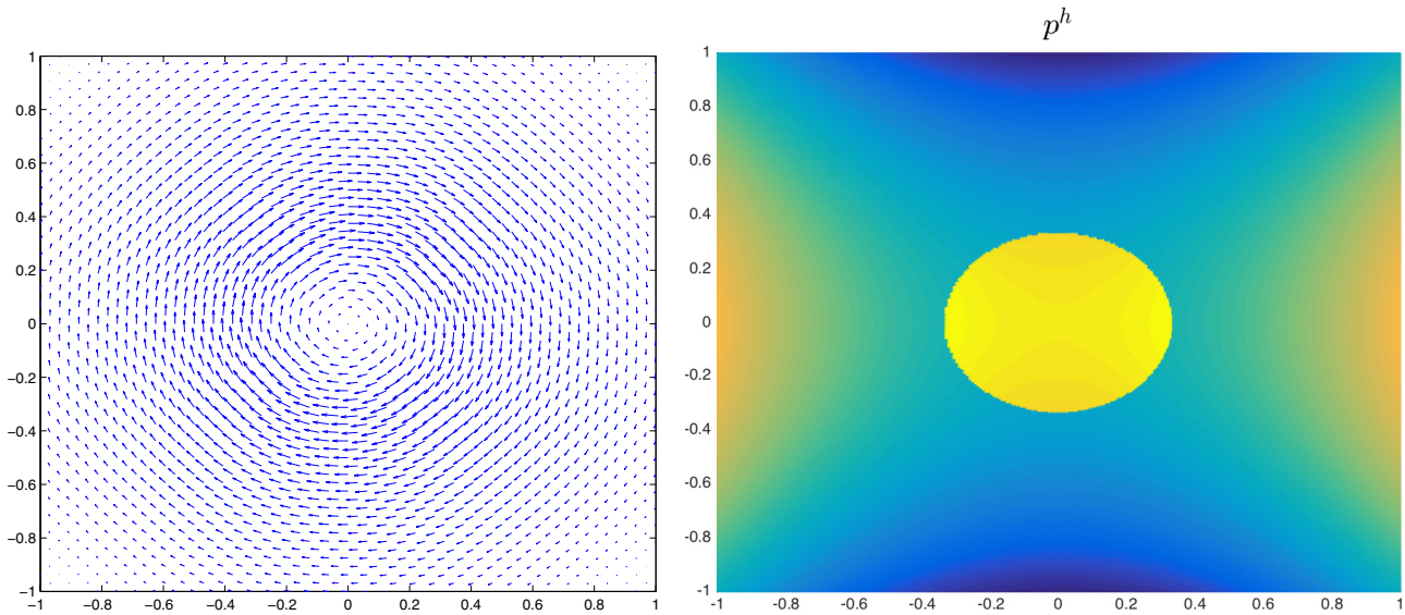
FIGURE 3. Plot of velocity ( left ) and discontinuous pressure ( right ).
