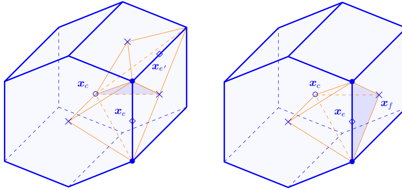
FIGURE 2. In blue. Left: Intra-cell sub-face f = \partial p_{e,c} \cap \partial p_{e',c} \in \mathfrak{F}_c . Right: Inter-cell sub-face f = \partial p_{e,c} \cap \partial p_{e',c'} \in \mathfrak{F}_f . (Color online)
