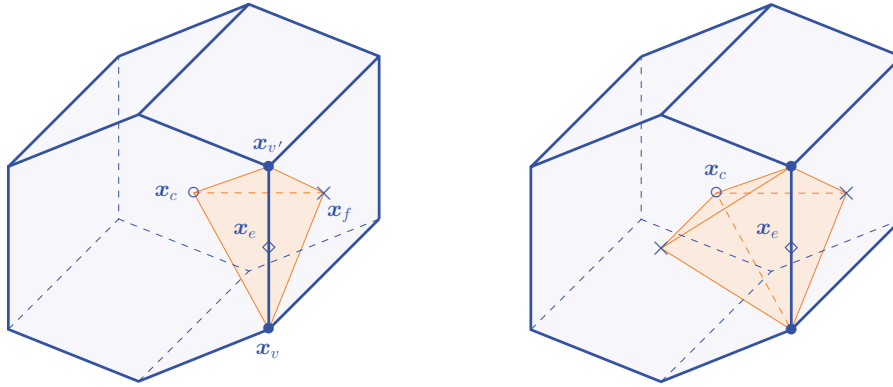
FIGURE 1. Left panel: Tetrahedron [x_v, x_{v'}, x_f, x_c] . Right panel: Local diamond \mathfrak{p}_{e,c} .
