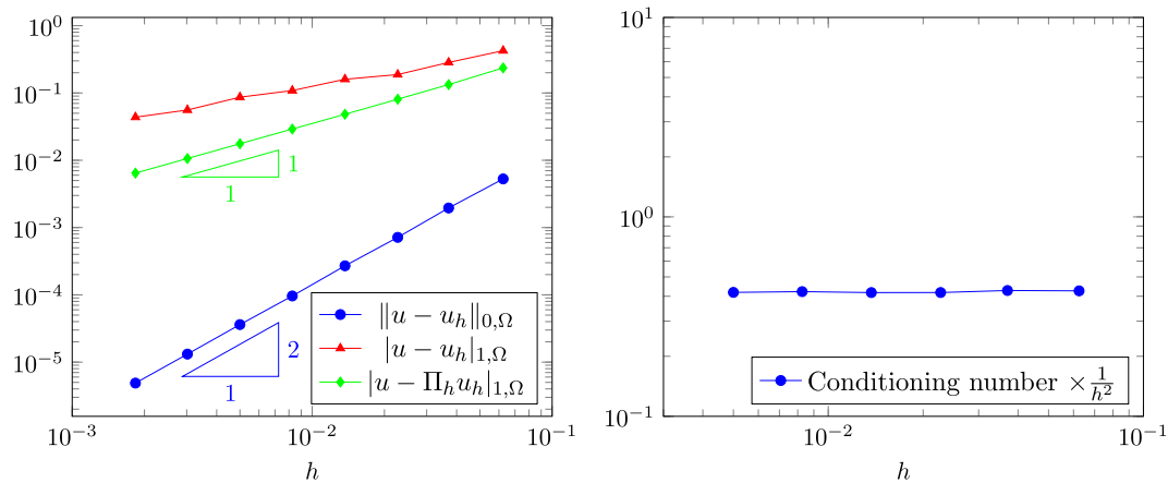
FIGURE 6. Errors (left) and conditioning number (right) for the alternative finite element scheme (3.3) on a sequence of meshes containing 10 degenerate cells with \rho_{K_i^{deg}} \sim h^2 . The H^1 norm is calculated both using the approximate solution u_h directly and extending it to the degenerate cells from the adjacent regular cells, as in (3.4). (Color online).
