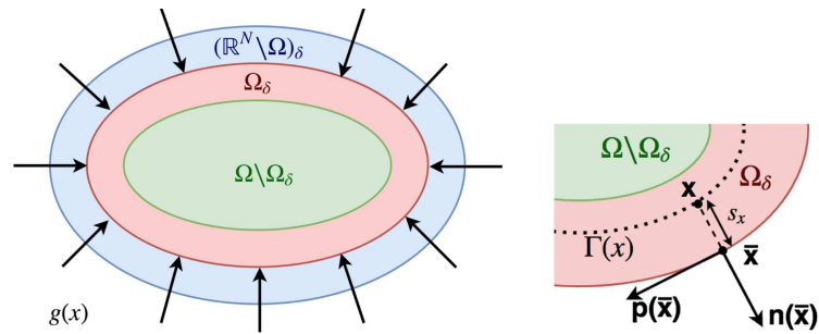
FIGURE 1. Left: notations for the domain, where \Omega is represented by the green and red regions together, and the nonlocal Neumann boundary condition is applied on the red region \Omega_\delta . Right: notations for the projection of point \mathbf{x} \in \Omega_\delta , the corresponding unit tangential vector \mathbf{p}(\bar{\mathbf{x}}) and the unit normal vector \mathbf{n}(\bar{\mathbf{x}}) .
