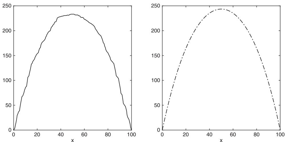
FIGURE 2. Left panel: FE-solution to the heterogeneous problem, and right panel: FE-solution to the corresponding homogenized problem. Both solutions are plotted along the line y = 55 . The fast oscillation in the left figure is clearly visible.
