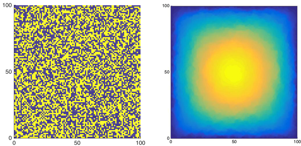
FIGURE 1. Left panel: a typical realization of the coefficient field \mathbf{a}(x) , with r = 100 (yellow corresponds to the value 1 and blue to the value 9). Right panel: corresponding solution.
