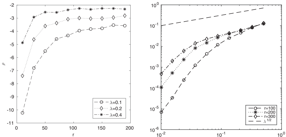
FIGURE 4. Left panel: averaged factor \rho as a function of r , for \lambda = 0.1, 0.2 , and 0.4 . Right panel: exponential of the averaged factor \rho as a function of \lambda for r = 100, 200 , and 300 . In all cases, the average is computed from ten simulation runs.
