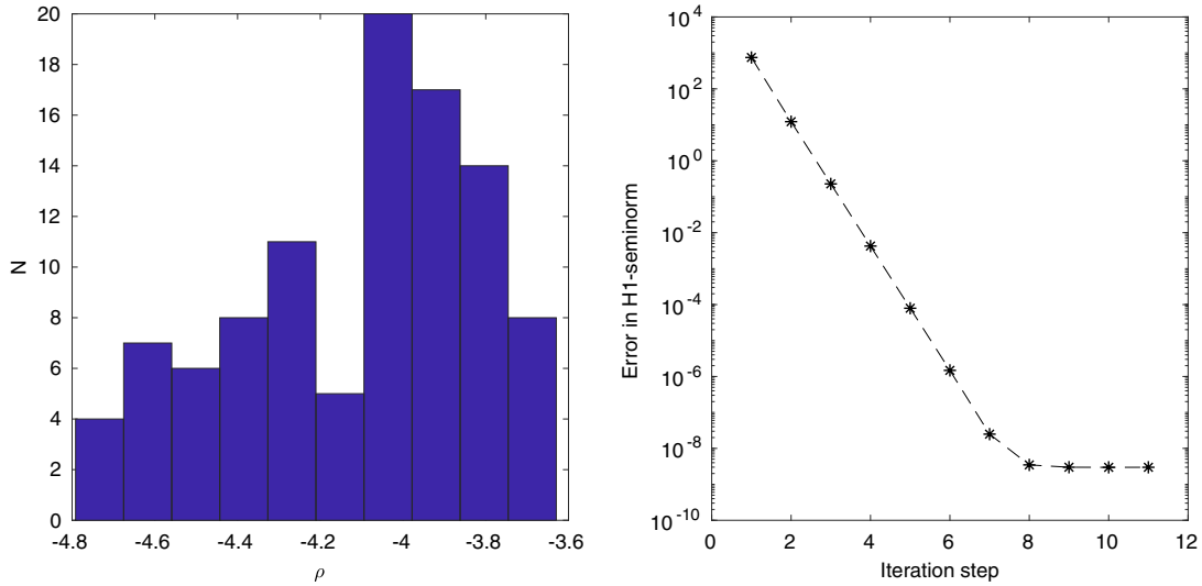
FIGURE 3. Left panel: empirical distribution of the factor \rho for \lambda = 0.1 and r = 100 , based on 100 runs. Right panel: error in the H^1 seminorm for r = 100 and \lambda = 0.1 , after each iteration. The method converges after 8 iterations.
