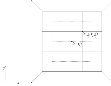
FIGURE 1. 2D overlapping cells formed by collapsing the staggered dual cells on two adjacent time levels to one time level.
