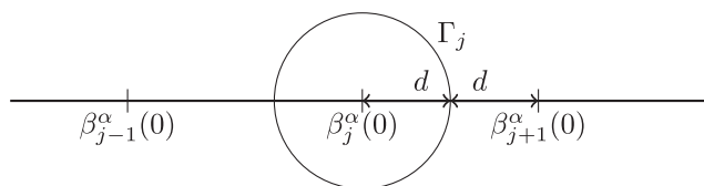
FIGURE 2. Schematic of \Gamma_j , d , \Sigma'(0) , and \Sigma''(0) .
