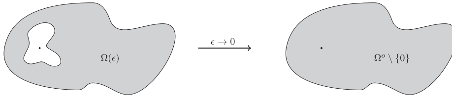
FIGURE 2. The perforated set \Omega(\epsilon) and the limiting punctured set \Omega^o \setminus \{0\} .
