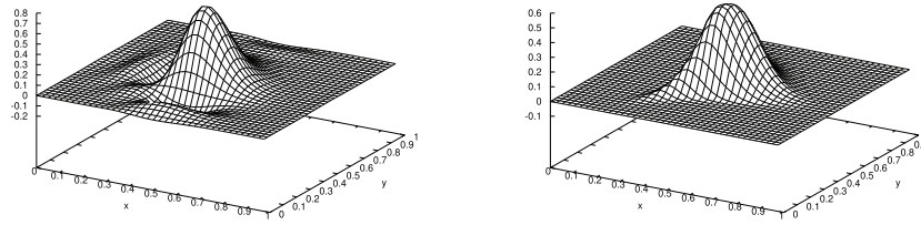
FIGURE 1. Advection of Gaussian. On the left calculated with the linear Lax–Wendroff scheme. On the right calculated with limitation of the fluxes. The maximum principle is not respected with the linear scheme. It is satisfied with the limitation procedure.
