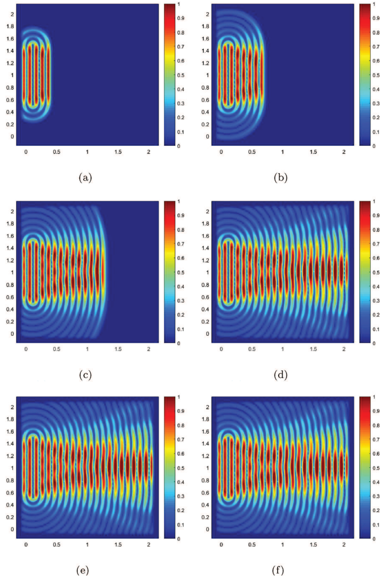
FIGURE 3. Snapshots of |H| field obtained with \tau = 10^{-12} s at 1000, 2000, 4000, 8000, 15 000, 20 000 time steps. (a) |H| at time step 1000. (b) |H| at time step 2000. (c) |H| at time step 4000. (d) |H| at time step 8000. (e) |H| at time step 15 000. (f) |H| at time step 20 000.
