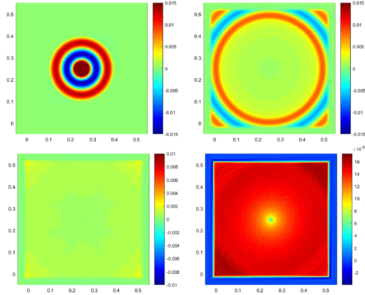
FIGURE 2. Snapshots of the magnetic field H : ( top left ) 200 steps; ( top right ) 500 steps; ( bottom left ) 700 steps; ( bottom right ) 1500 steps.
