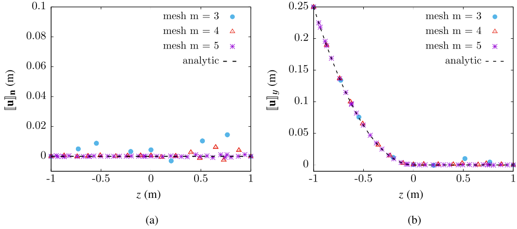
FIGURE 9. (a) Nodal normal jumps \llbracket \mathbf{u}_{\mathcal{D}} \rrbracket_{\mathcal{D}, \mathbf{n}} and (b) nodal tangential jumps \llbracket \mathbf{u}_{\mathcal{D}} \rrbracket_{\mathcal{D}, y} , along the line x = y = 0 as functions of z for the discrete solutions on the Hexa-cut meshes with 2^{3m} cells, m = 3, 4, 5 . Test case of Section 6.2.
