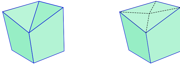
FIGURE 7. Example of randomly perturbed Cartesian cell with non planar faces: hexahedral cell with a non planar face cut into two triangles (left, denoted by Hexa-cut) or four triangles using the isobarycenter of the face nodes (right, denoted by Hexa-bary). Note that in the Hexa-bary case, the displacement at the isobarycenter is eliminated by linear combination of the displacements at the face nodes as detailed in Remark 3.1.
