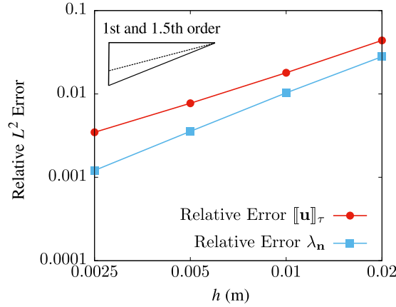
FIGURE 6. Convergence of the relative L^2 error of \llbracket \mathbf{u} \rrbracket_\tau - \llbracket \mathbf{u}_D \rrbracket_{D,\tau} and of \lambda_n - \lambda_{D,n} away from the tip, as a function of the size of the largest fracture face denoted by h . Test case of Section 6.1.
