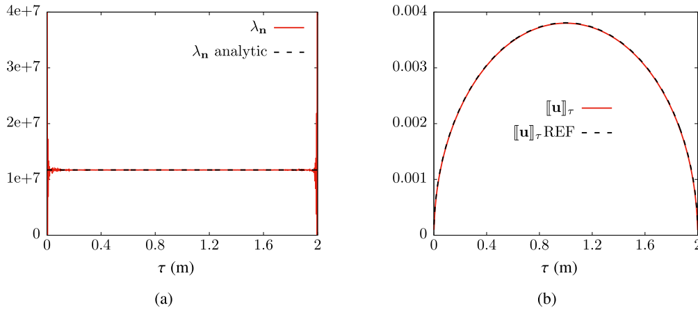
FIGURE 5. Comparison between the numerical and analytical solutions on the finest mesh (with 800 fracture faces), for (a) \lambda_n , and (b) [[\mathbf{u}]]_\tau ; example of Section 6.1.
