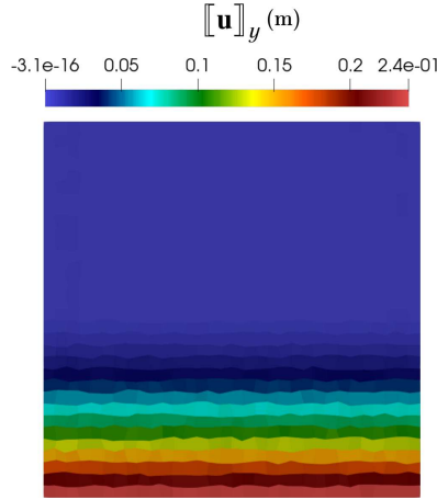
FIGURE 10. Face-wise constant non-zero tangential component jump \llbracket \mathbf{u}_{\mathcal{D}} \rrbracket_{\mathcal{D}, y} on \Gamma obtained on the Hexa-cut mesh with 2^{3m} cells, m = 5 . Test case of Section 6.2.
