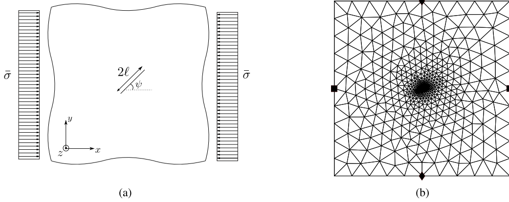
FIGURE 4. (a) unbounded domain containing a single fracture under uniform compression, and (b) mesh including nodes for boundary conditions (◆: u_x = 0 , ■: u_y = 0 ), for the example of Section 6.1.
