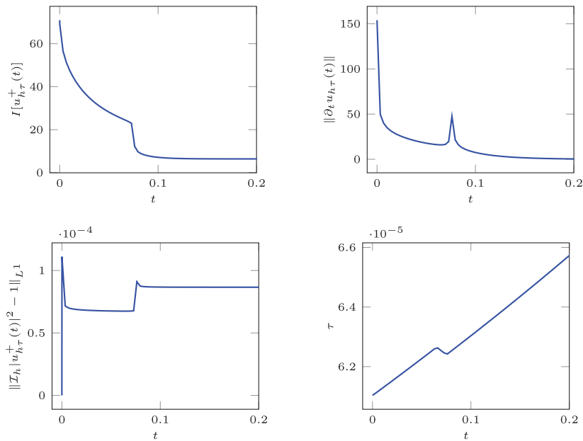
FIGURE 4. Evolution in [0, 1/5] of the energy ( top-left ), the L^2 -norm of the update ( top-right ), the constraint violation L^1 -error ( bottom-left ), and the step size ( bottom-right ) for the approximations generated by the midpoint method with adaptively adjusted step size ( \tau_1 = 2^{-14} ).
