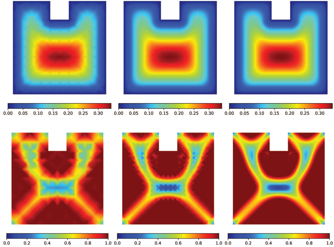
FIGURE 3. The first three discrete solutions u_h (top) and gradient magnitudes |\nabla u_h| (bottom) for the nonconvex example.
