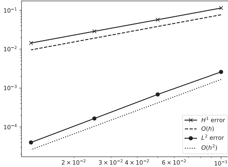
FIGURE 4. The error between u_h and a reference solution as a function of the mesh parameter h for the convex example. The reference solution is obtained using a quadratic finite element method on a suitably refined mesh.
