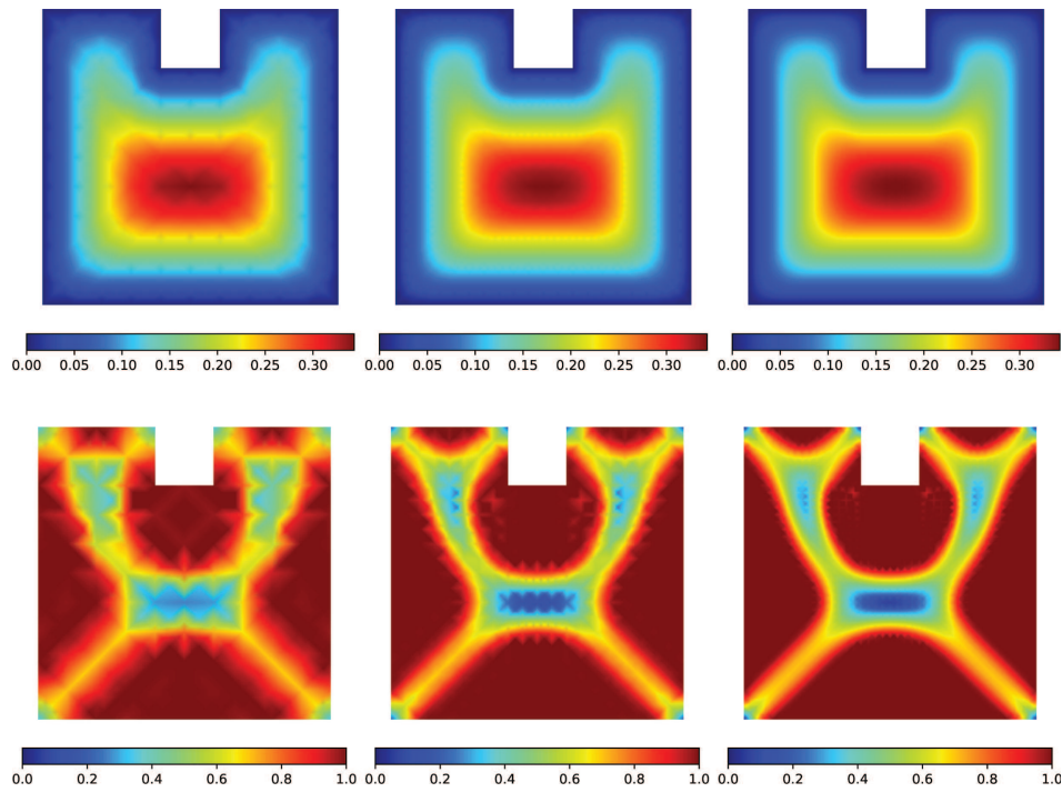
FIGURE 8. The first three discrete solutions u_h ( top ) and gradient magnitudes |\nabla u_h| ( bottom ) for the nonconvex example using the method of [8].
