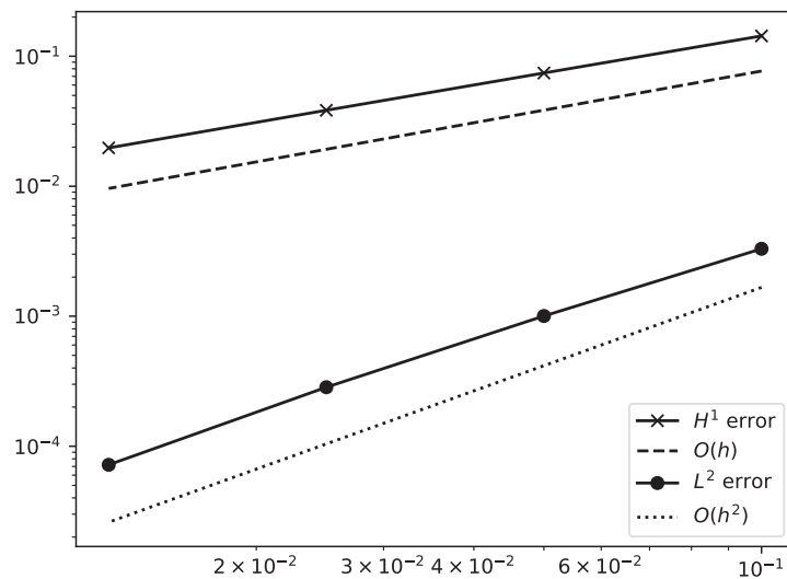
FIGURE 9. The error between u_h and a reference solution as a function of the mesh parameter h for the nonconvex example using the method of [8].
