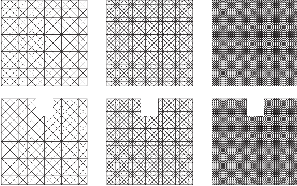
FIGURE 1. The first three meshes for the convex ( top ) and nonconvex ( bottom ) examples from the uniform mesh sequences. The side length of the larger square is 1 while the smaller square in the nonconvex example has a side length of 0.2.
